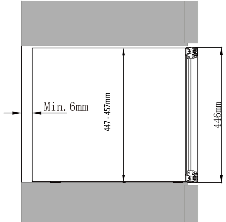
Side View
