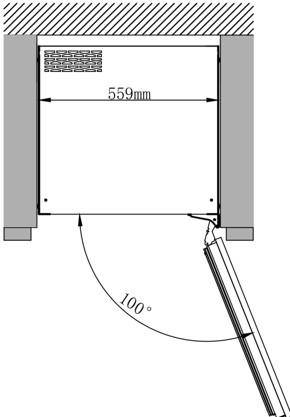
Top View
